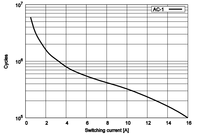
CIM2, CIM2R - Electrical endurance
